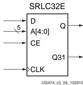
Figure 3-4: 32-Bit Shift Register
