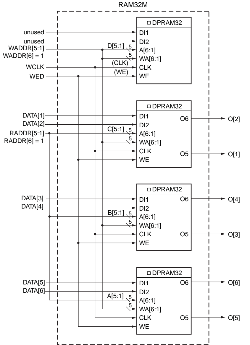
Figure 2-7: 32 X 6 Simple Dual Port Distributed RAM (RAM32M)
